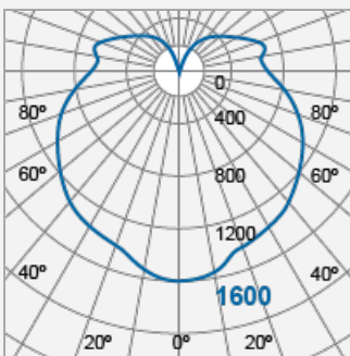
Integrated LED Luminaire FOB61100v1-pl
